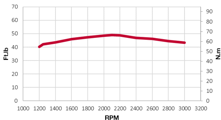
TORQUE
